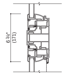
Vertical Section
