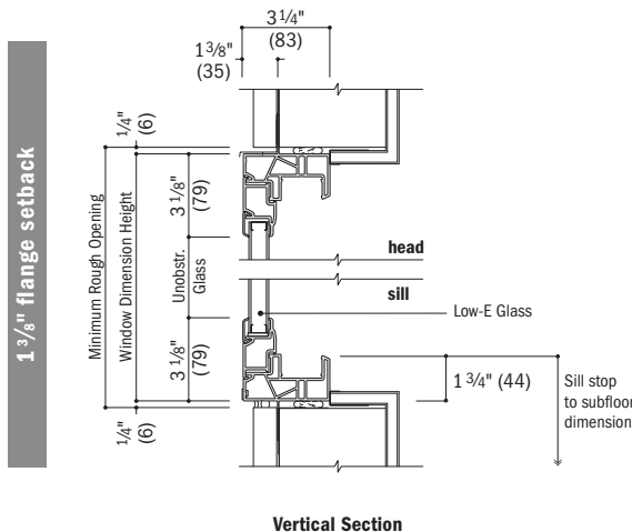
Vertical Section
