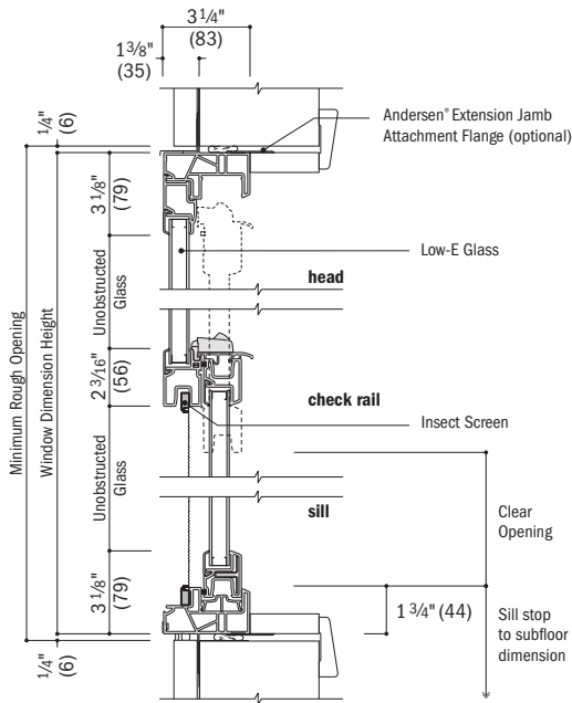
Vertical Section
