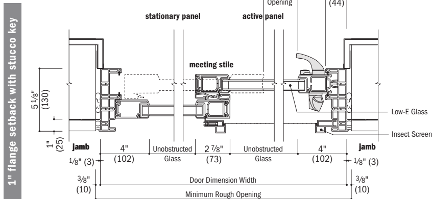
Horizontal Section stucco exterior
