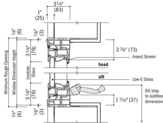
Vertical Section
