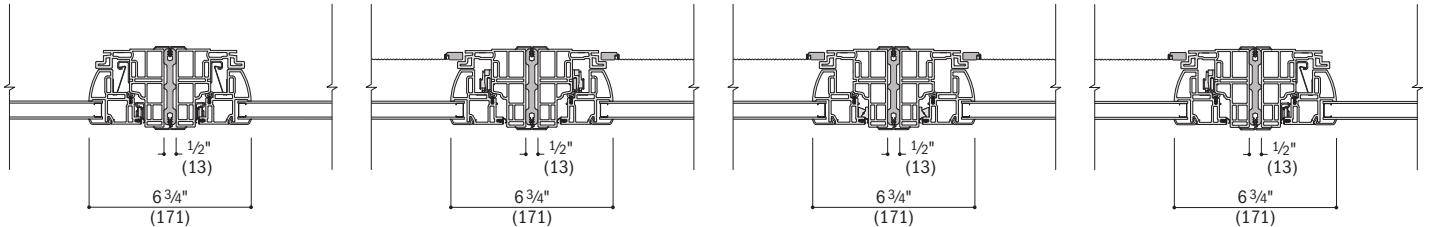
Casement to Casement (stationary jamb to stationary jamb)
