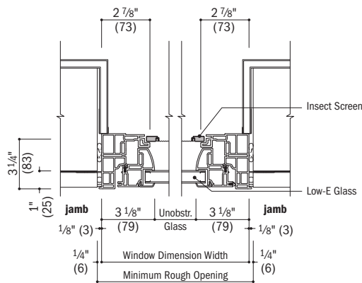
Horizontal Section
