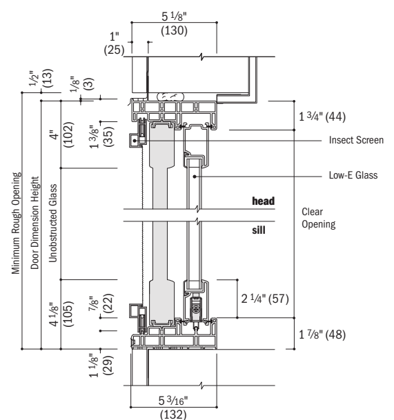
Vertical Section stucco exterior
