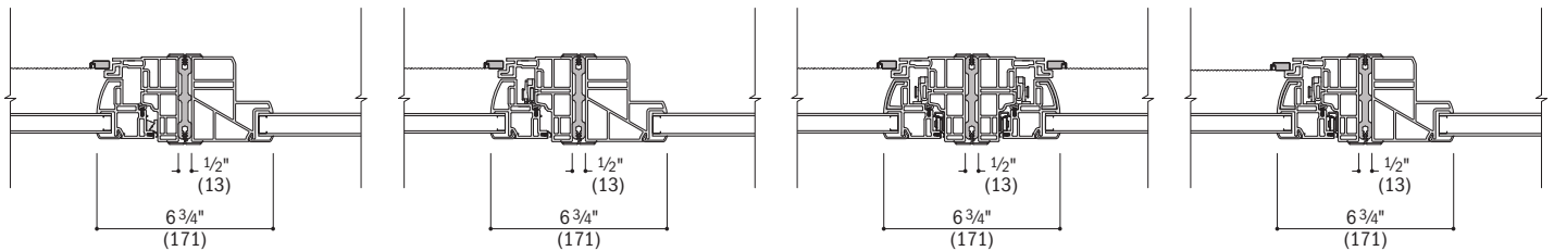
Casement to Picture/Single Transom (casement hinge jamb)
