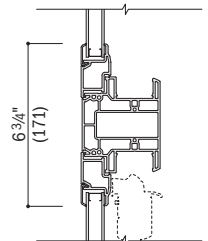
Vertical Section Transom over Single-Hung
