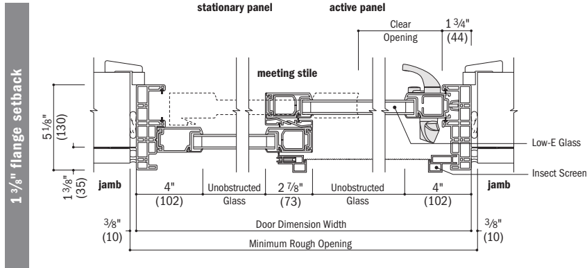
Horizontal Section
