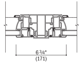
Horizontal Section
