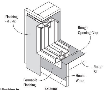
Exterior
