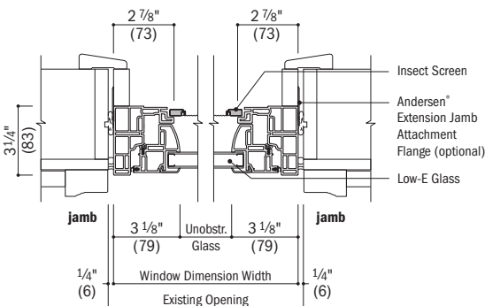
Horizontal Section
