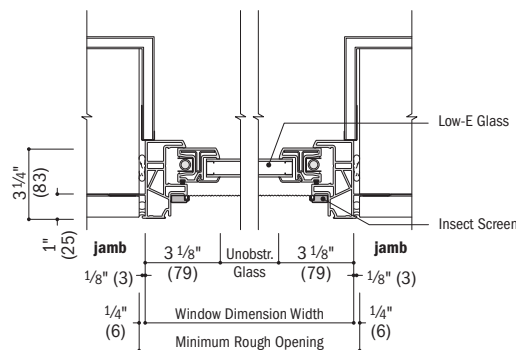
Horizontal Section Arch Single-Hung - stucco exterior
