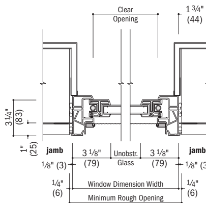
Horizontal Section stucco exterior
