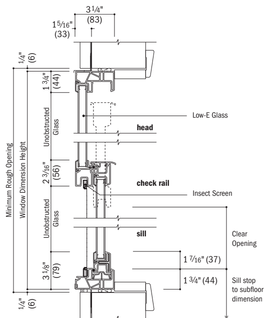
Vertical Section Arch Single-Hung
