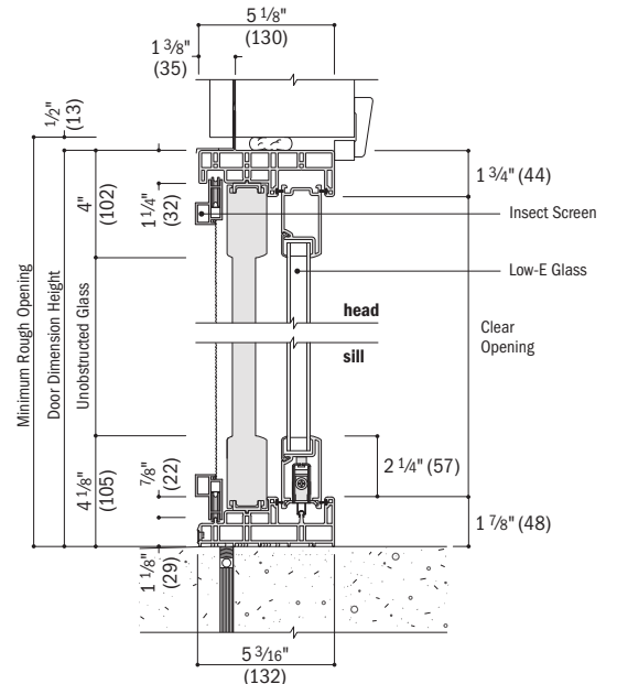
Vertical Section
