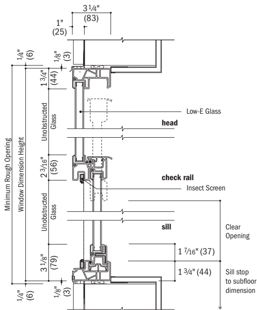
Vertical Section Arch Single-Hung - stucco exterior
