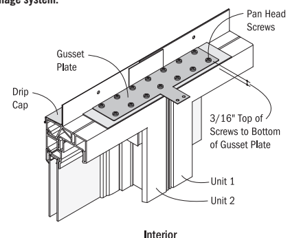
Interior
