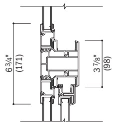
Horizontal Section Picture over Gliding
